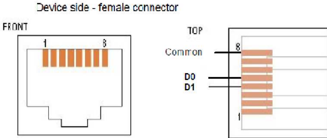
Figure 24: 2W- MODBUS on RJ45 connector ( required pin-out )
