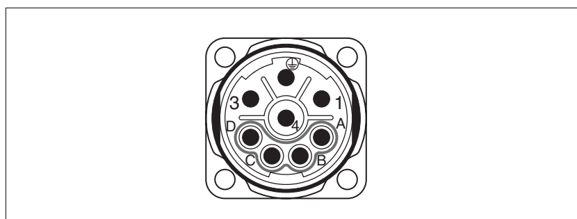
Figure 13: Pin assignment motor connection M23
