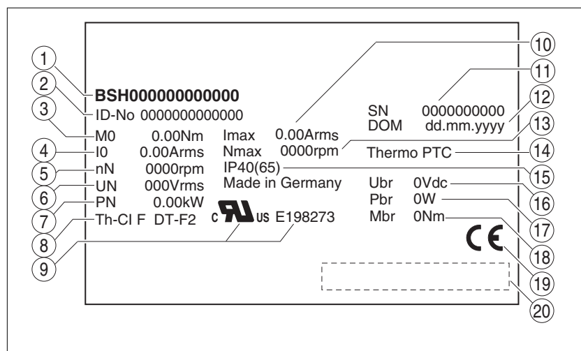
Figure 1: Nameplate
