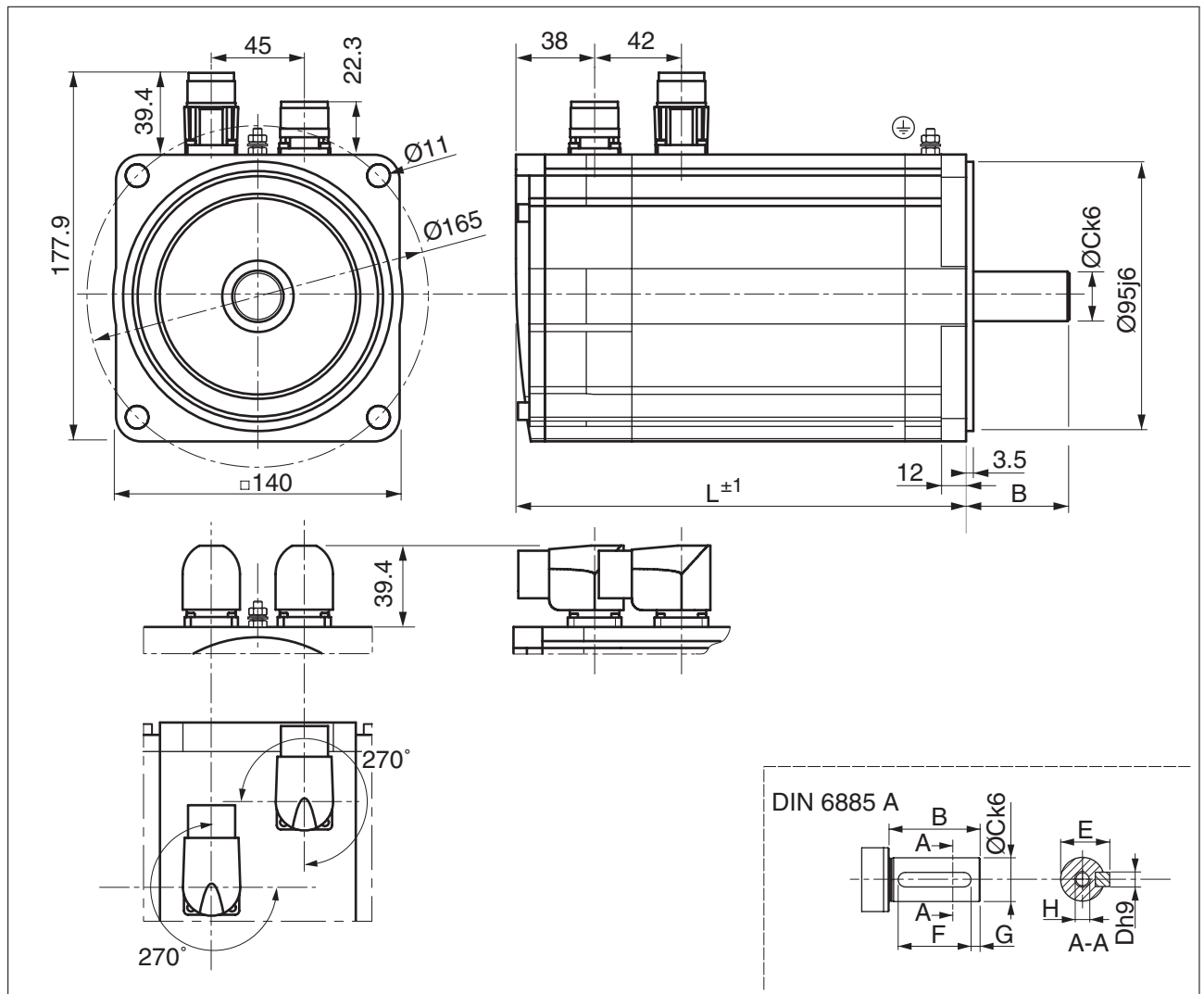
Figure 5: Dimensions BSH1401 (M, P, T); BSH1402 (M, P); BSH1403 (M, P); BSH1404 (M)
