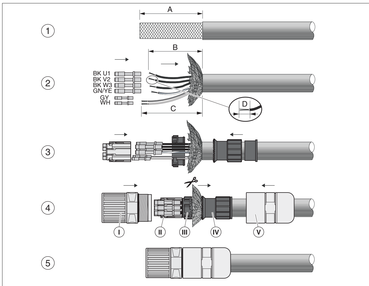
Figure 18: Assembling motor cables with M23 motor connector
