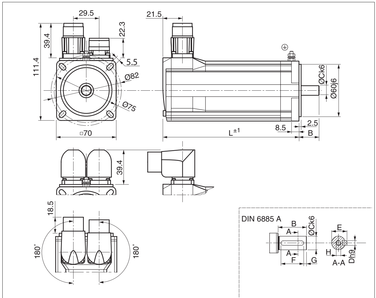
Figure 3: Dimensions BSH070
