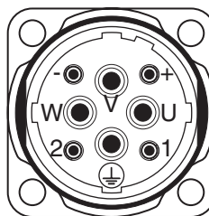
Figure 14: Pin assignment motor connection M40
