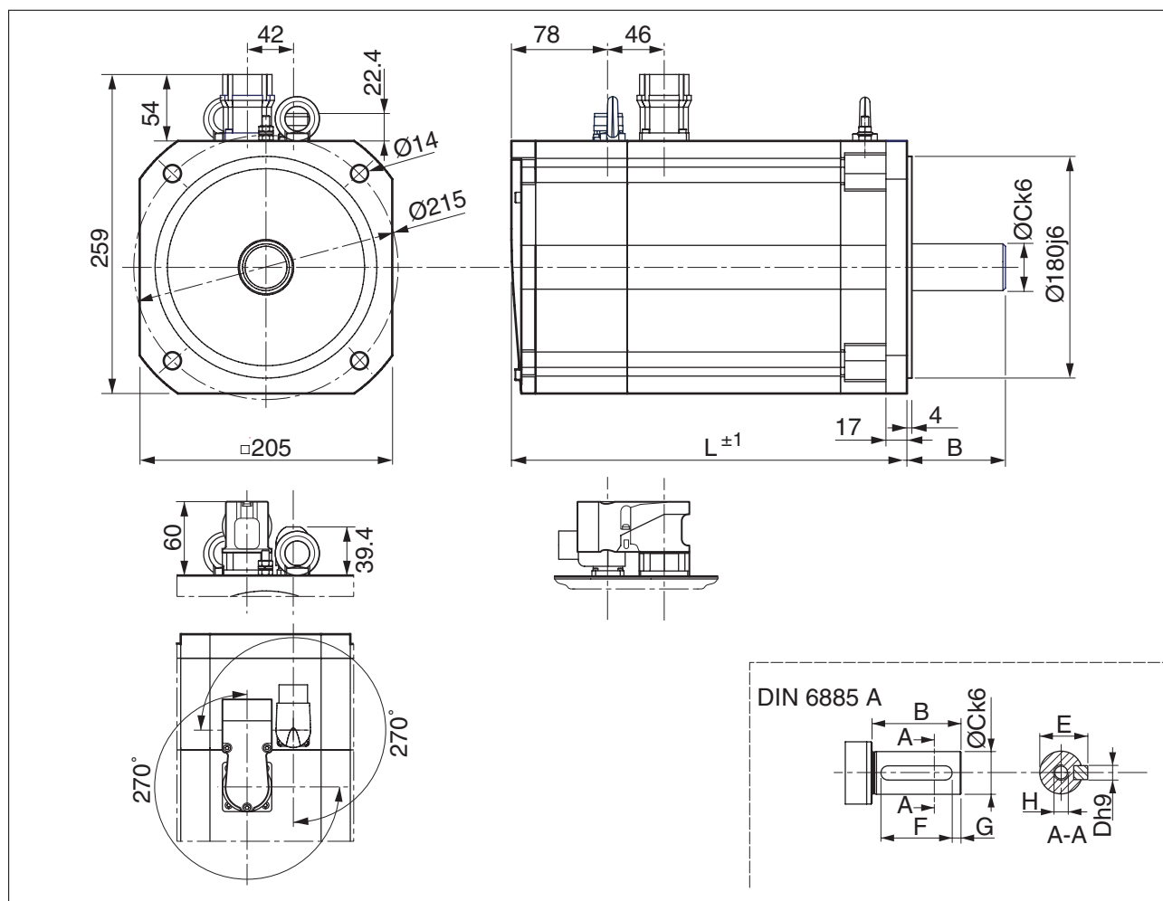
Figure 7: Dimensions BSH205 with connector
