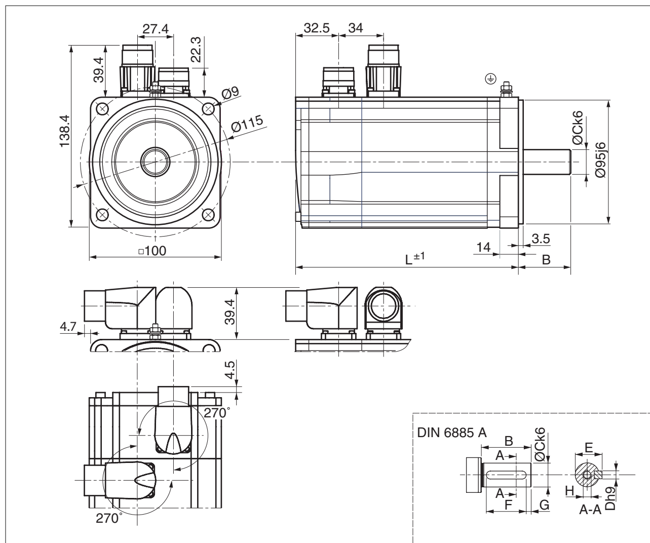
Figure 4: Dimensions BSH100
