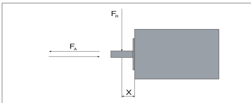
Figure 9: Shaft load
