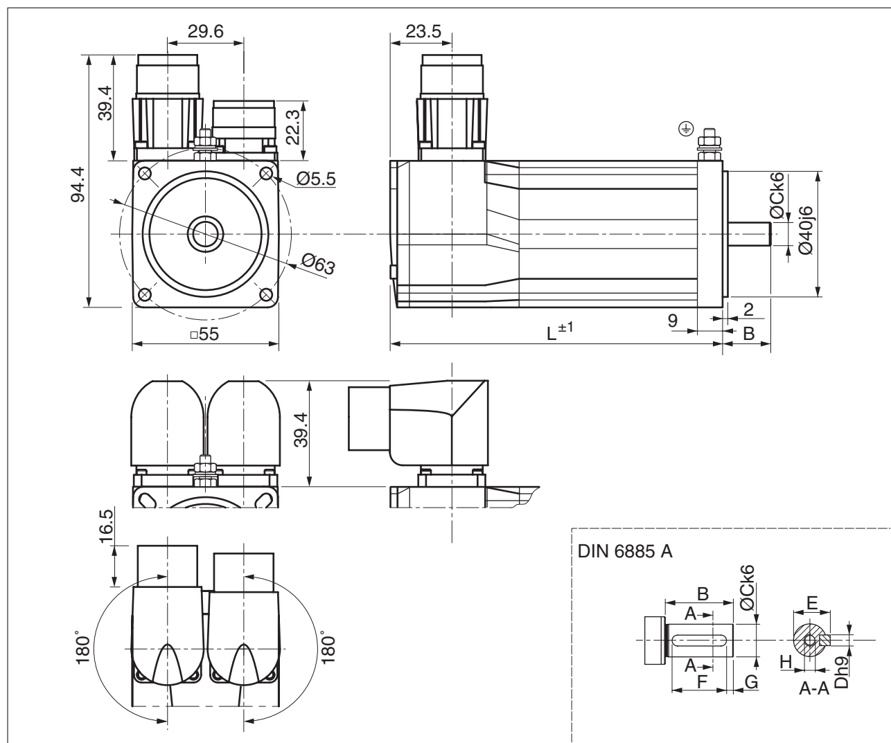
Figure 2: Dimensions BSH055
