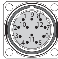
Figure 15: Pin assignment encoder connector
