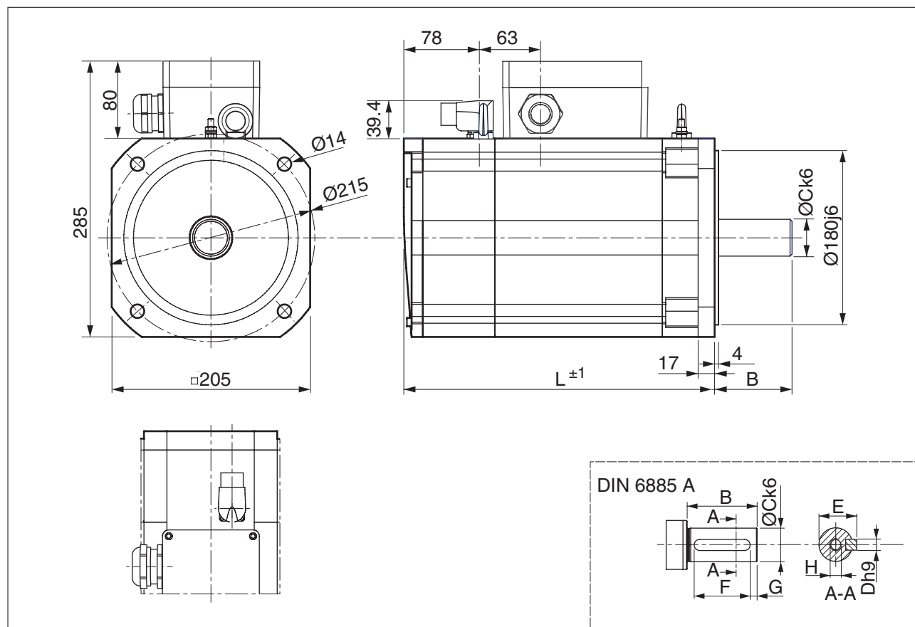
Figure 8: Dimensions BSH205 with terminal box
