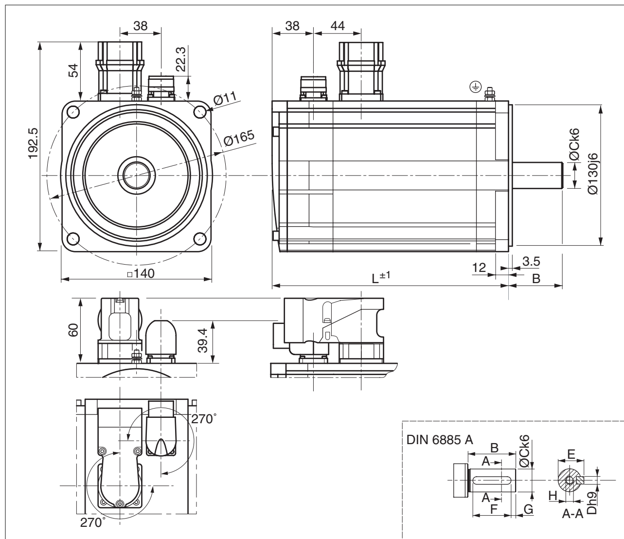
Figure 6: Dimensions BSH1402 (T); BSH1403 (T); BSH1404 (P)
