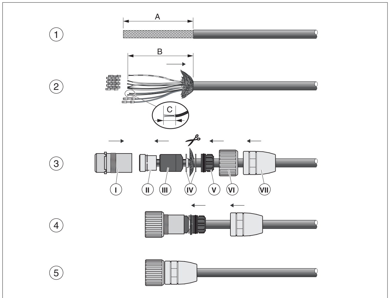
Figure 17: Assembling encoder cables with M23 encoder connector
