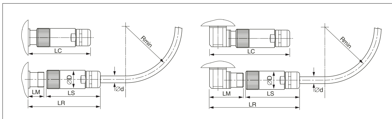
Figure 10: Connector installation space
